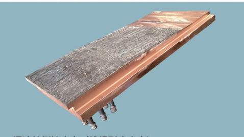
闪速炉侧墙水套（堆焊耐磨合金） side wall water jacket of flash furnace (welded wear-resistant alloy)
