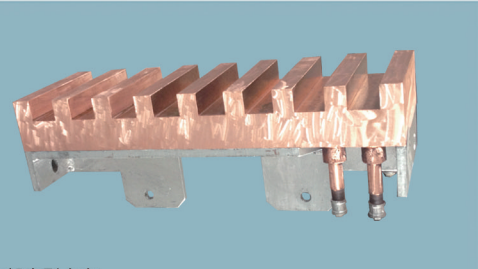
闪速炉反应塔底部齿型水套 toothed water jacket at the bottom of the flash furnace reaction tower
