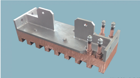
闪速炉反应塔底部齿型水套 toothed water jacket at the bottom of the flash furnace reaction tower
