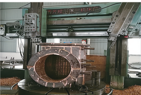
立式车床 VERTICAL LATHE
