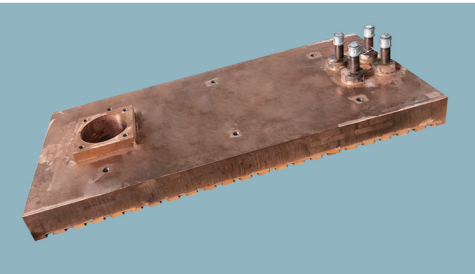
侧吹炉风口铜水套 gas-inlet copper water jacket of side blow furnace
