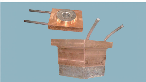
闪速炉放铜口水套（堆焊耐磨合金） copper outlet water jacket (welded wear-resistant alloy)
