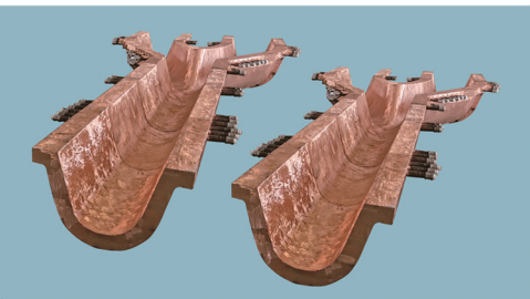
侧吹炉溜槽 launder of side blow furnace
