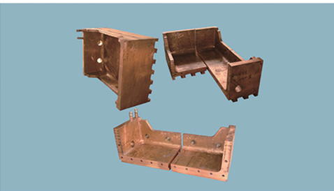
基夫赛特炉框架铜水套 frame copper water jacket of Kivcet furnace
