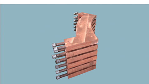
顶吹炉平水套 flat water jacket of top blow furnace
