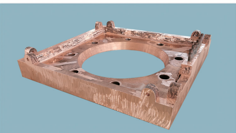
闪速炉加料口底座铜水套 feeding base copper water jacket of flash furnace
