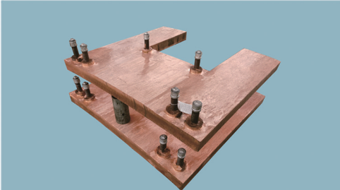
圆形镍铁电炉立水套 vertical water jacket of circular ferro-nickel furnace
