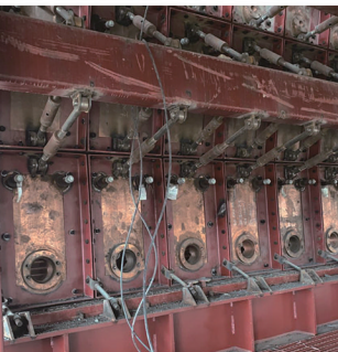
铜冶炼侧吹炉铜水套现场安装照片 photo of copper water jacket installation in side blow furnace
