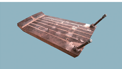
艾萨炉铜水套 copper water jacket of Isa furnace
