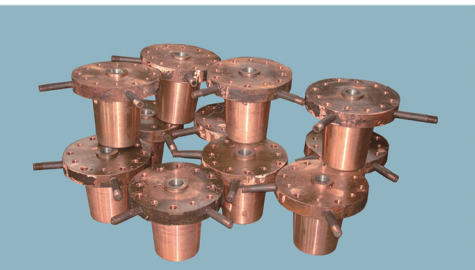
侧吹炉风嘴头 tuyere of side blow furnace
