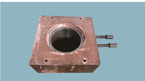
底吹炉内孔镶钢放出口铜水套 outlet copper water jacket with steel sleeve of bottom blow furnace
