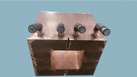
圆形镍铁电炉放铁、放渣口铜水套 copper water jacket for iron and slag outlet of circular ferro-nickel furnace
