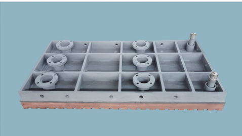
烟化炉异种材料复合水套 different material composite water jacket of fuming furnace
