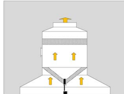
Double stage, with downward coned 1 st stage Coalescer
