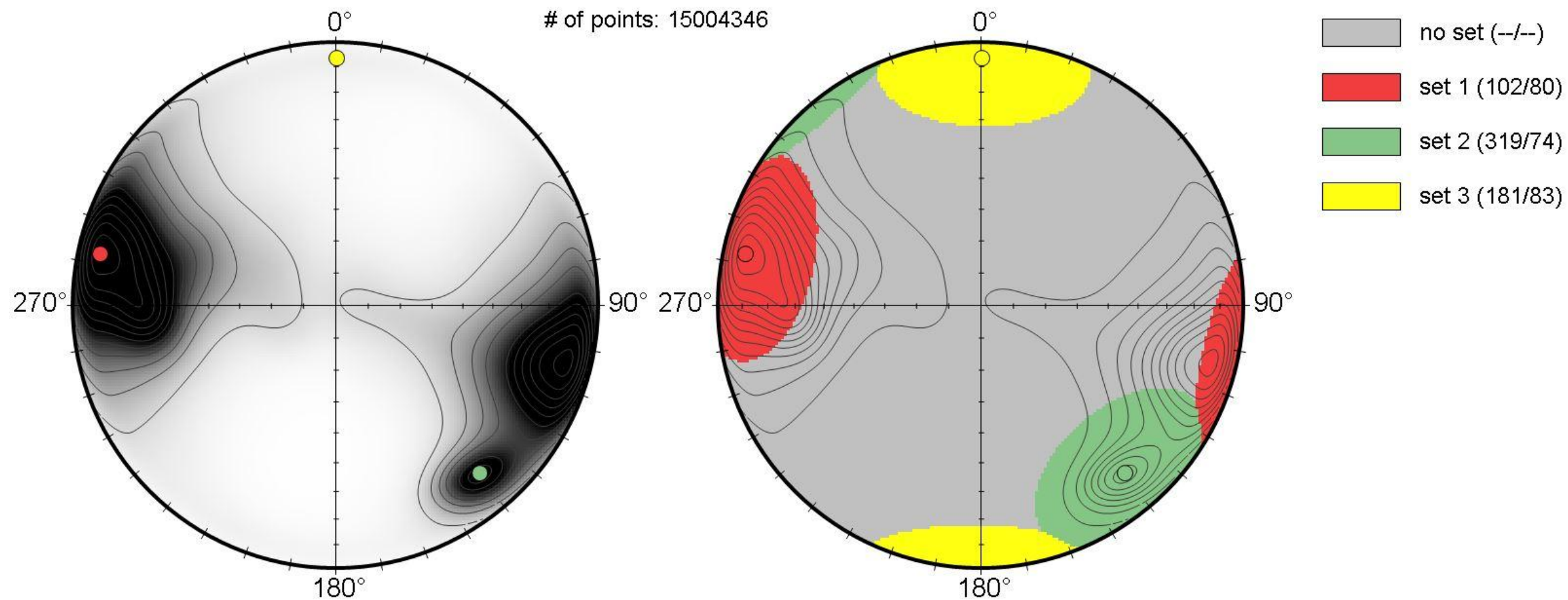
Stereonet Plot Through Mesh
